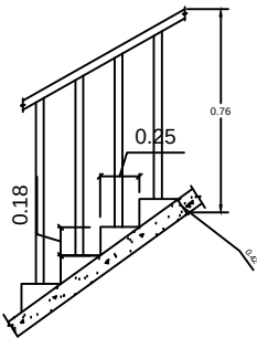
SECTION OF STAIRCASE SCALE 1:100
