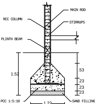
COLUMN DETAILS SCALE 1:100
