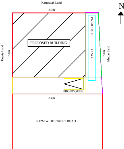
SITE PLAN
