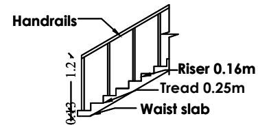
STAIRCASE DETAILS
