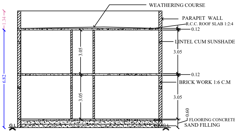
Section on-"AA"
