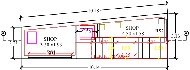
Ground Floor
