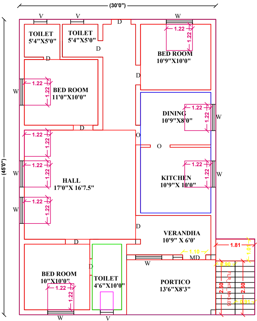
FLOOR-GROUND
