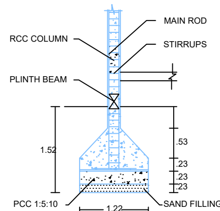
COLUMN DETAILS
