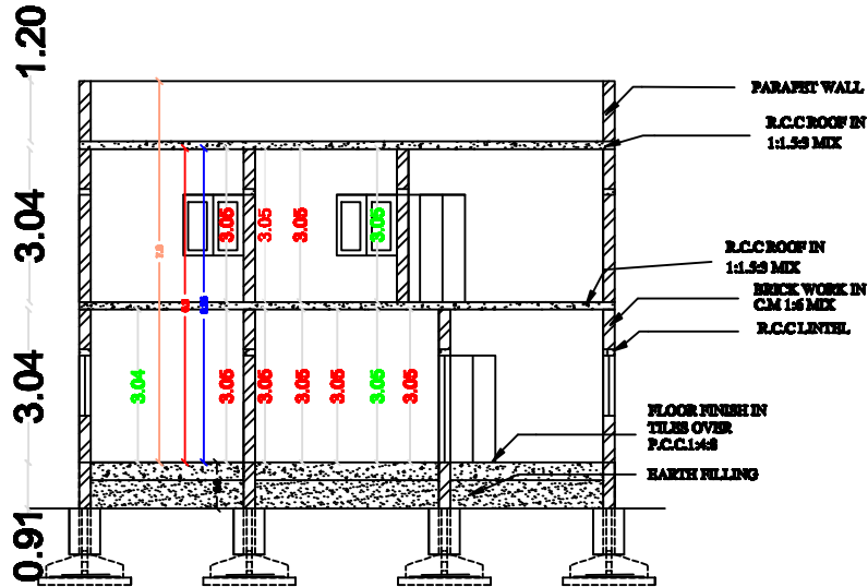
SECTION AB
