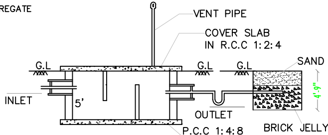
SECTION-AB
