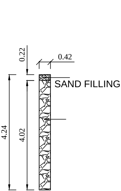
DETAILS OF PERCOLATION PIT
