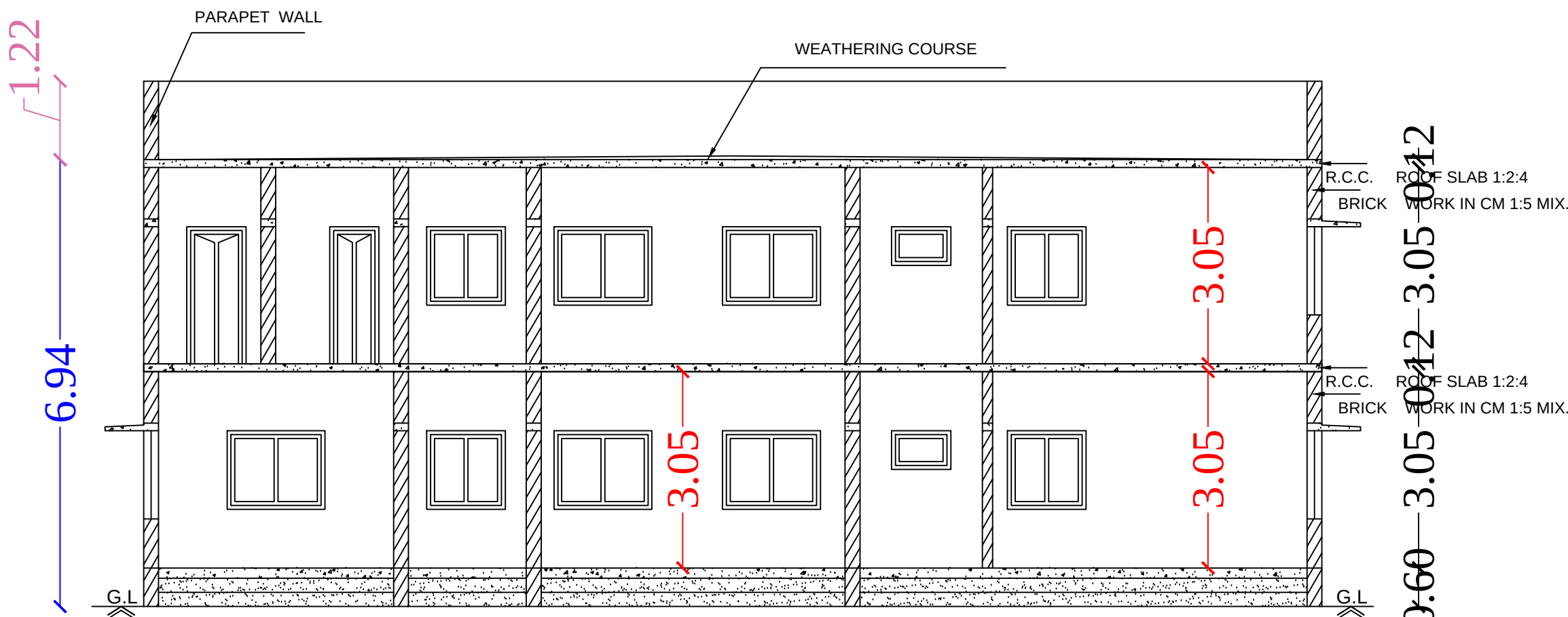
Section on-"AA"
