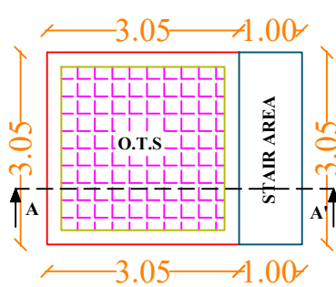
PRO TERRACE FLOOR
