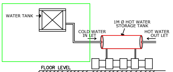
Solar Hot Water System Detail
