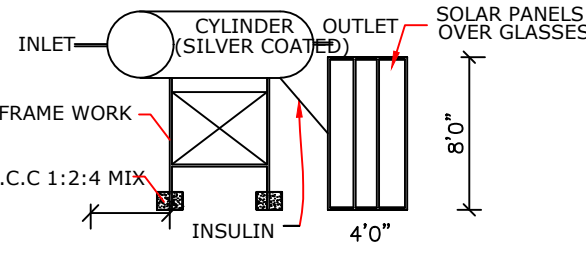
Waste Water Recycle Unit Not To Scale
