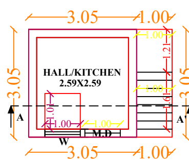
PRO GROUND FLOOR
