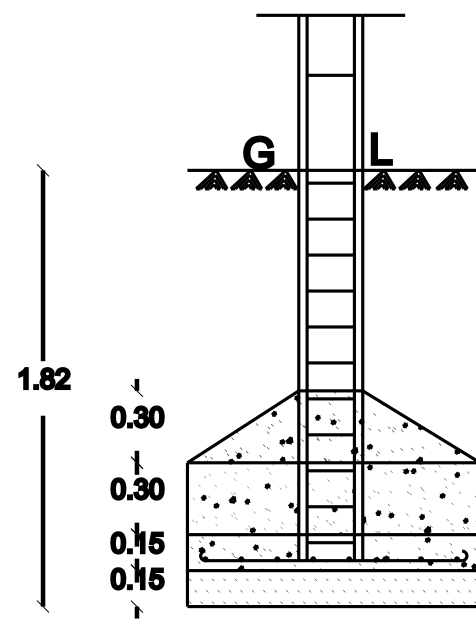
SECTION
