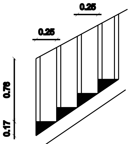
DETAILS OF STAIR CASE
