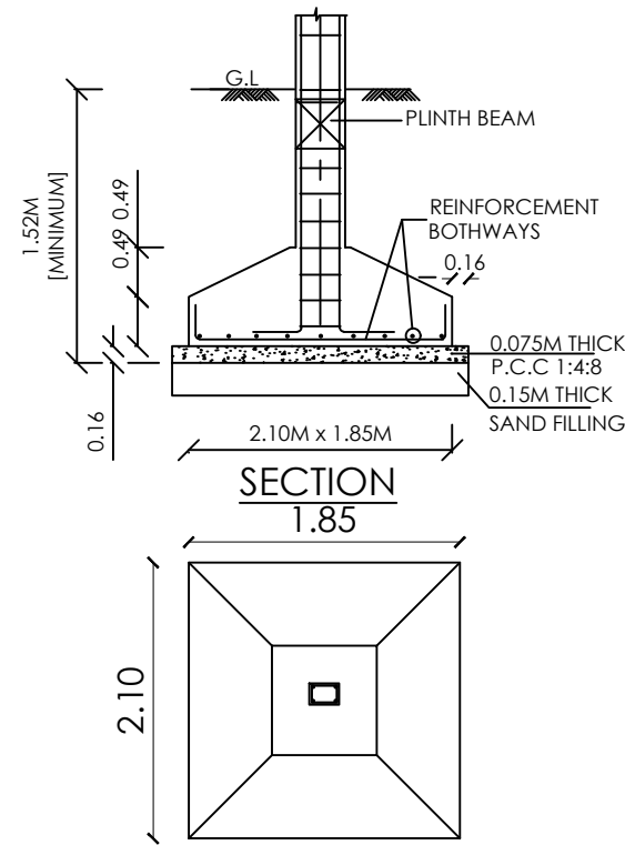
FOUNDATION DETAILS
