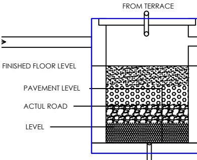
II Detail
