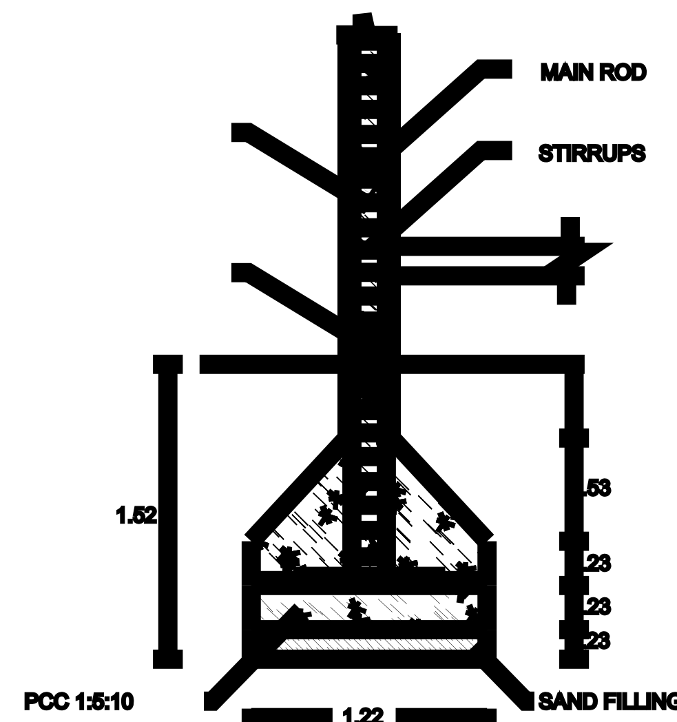
COLUMN DETAILS
