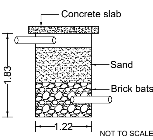
RAIN WATER STORAGE
