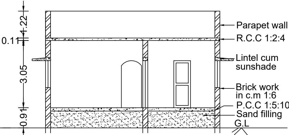
CROSS SECTION ON"AB"
