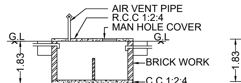
SEPTICTANK DETAILS
