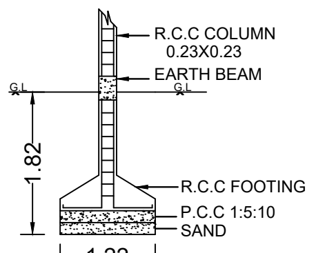
FOUNDATION DETAILS
