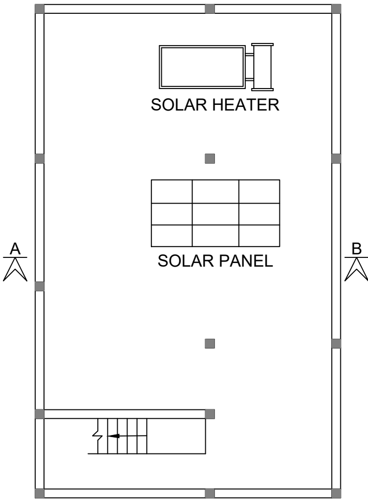
TERRACE PLAN
