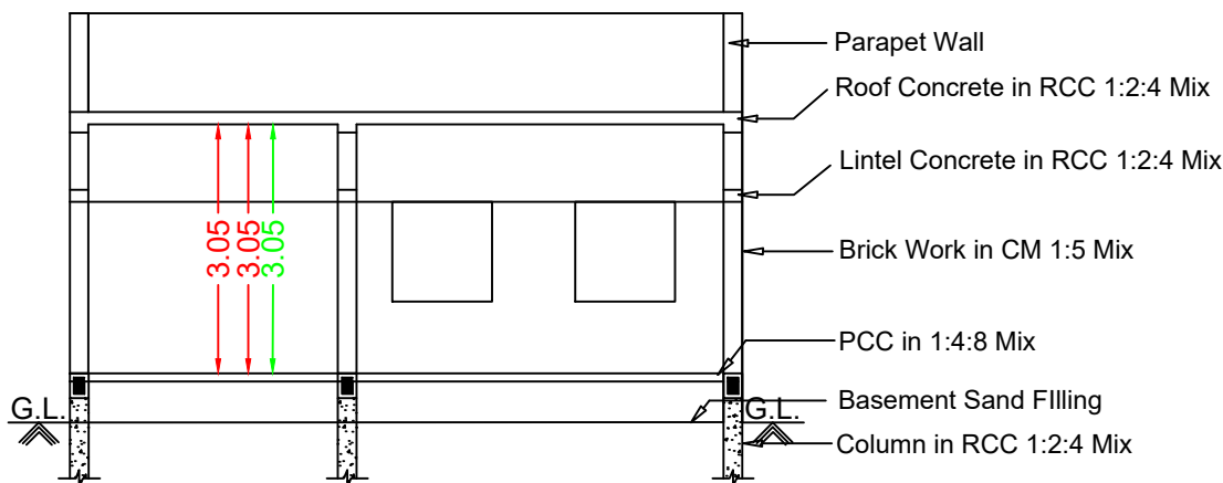
Section RR
