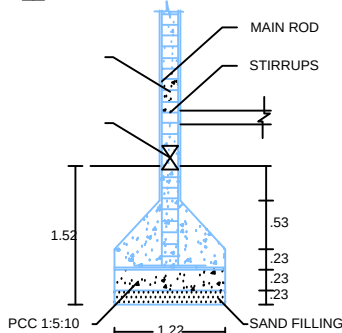
COLUMN DETAILS
