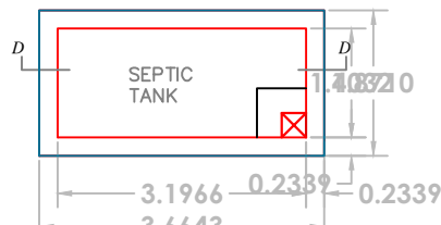
PLAN OF SEPTIC TANK SCALE 1"=2'0"
