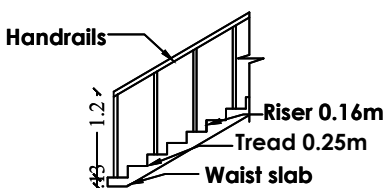
STAIRCASE DETAILS
