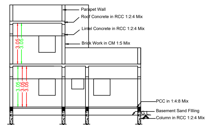
Section RR
