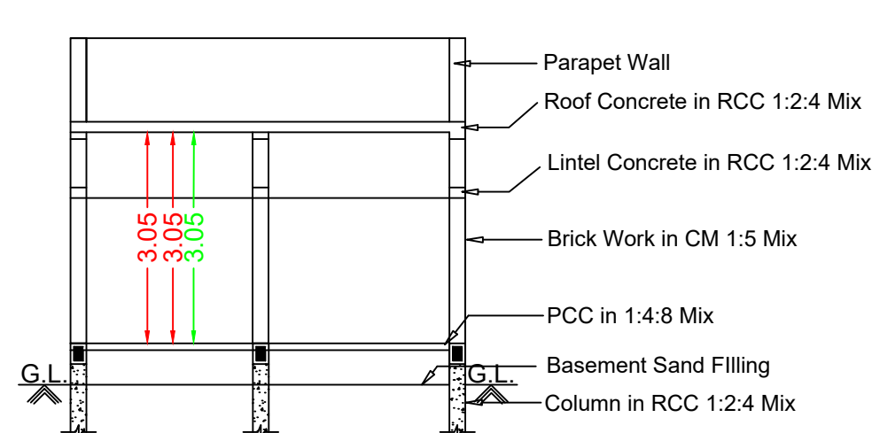
Section RR
