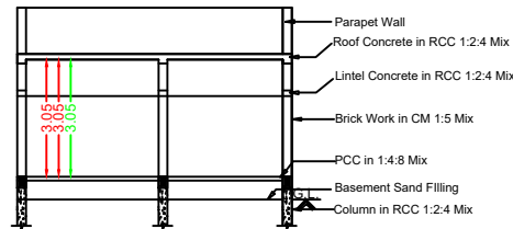
Section RR
