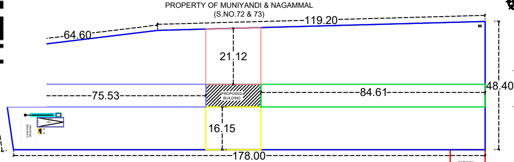
SITE PLAN (1:100)
