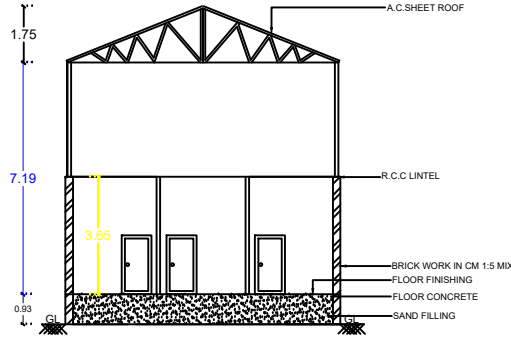
SECTION A1-A1
