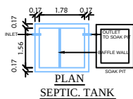
PLAN SEPTIC. TANK
