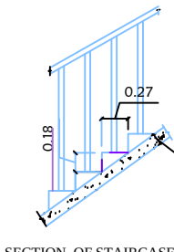
SECTION OF STAIRCASE
