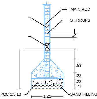
COLUMN DETAILS
