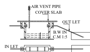
DETAILS OF SEPTIC TANK & D-TRENCH
