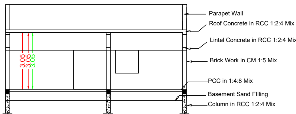
Section RR
