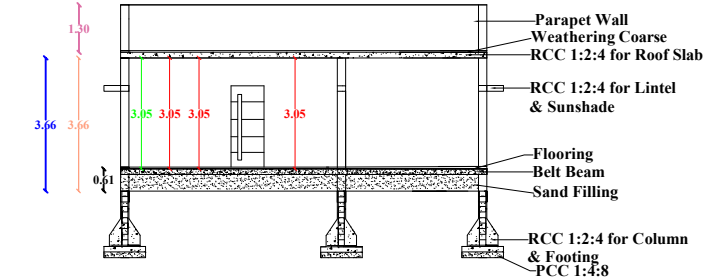
SECTION AB
