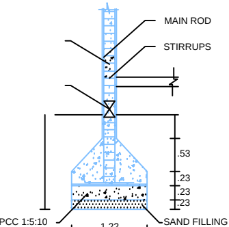
COLUMN DETAILS
