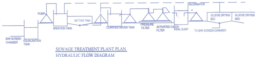
SEWAGE TREATMENT PLANT PLAN HYDRAULIC FLOW DIAGRAM
