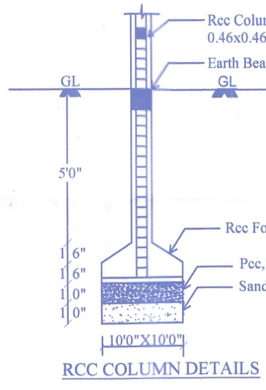
RCC COLUMN DETAILS
