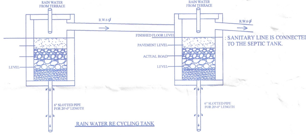
RAIN WATER RECYCLING TANK
