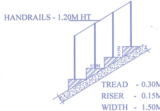
STAIRCASE DETAILS
