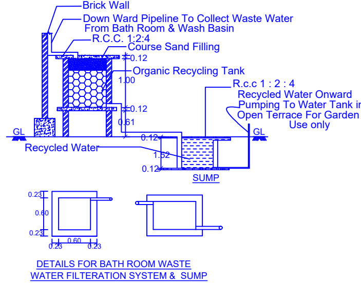
DETAILS FOR BATH ROOM WASTE WATER FILTRATION SYSTEM & SUMP
