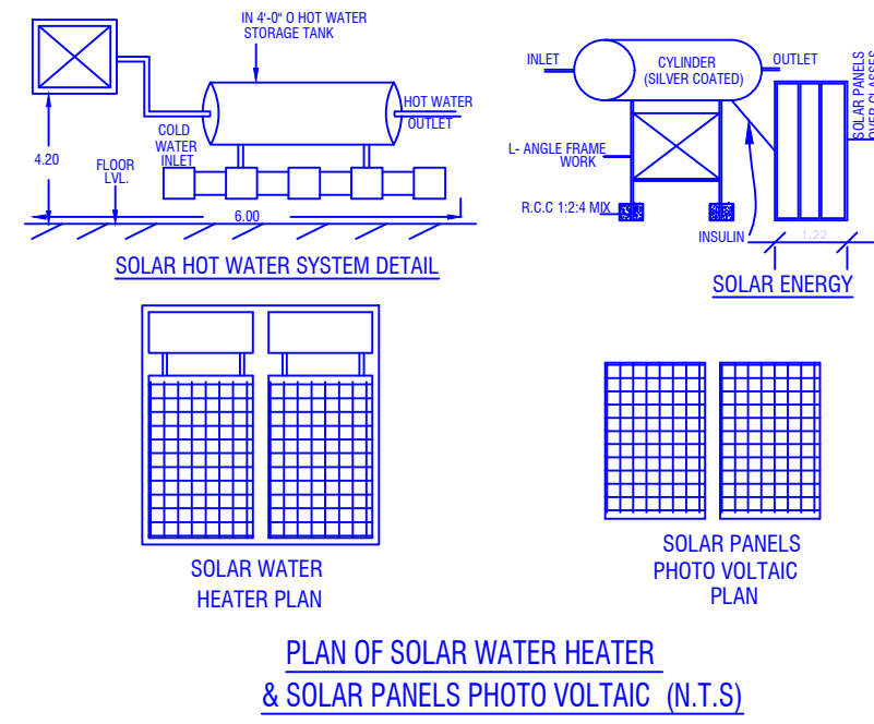
PLAN OF SOLAR WATER HEATER & SOLAR PANELS PHOTO VOLTAIC (N.T.S)
