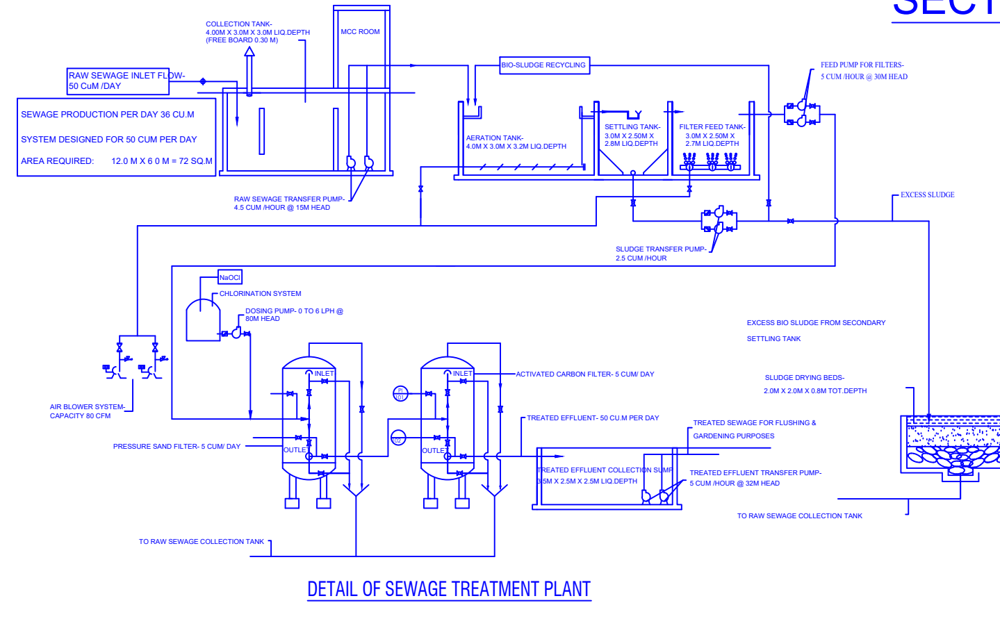
DETAIL OF SEWAGE TREATMENT PLANT
