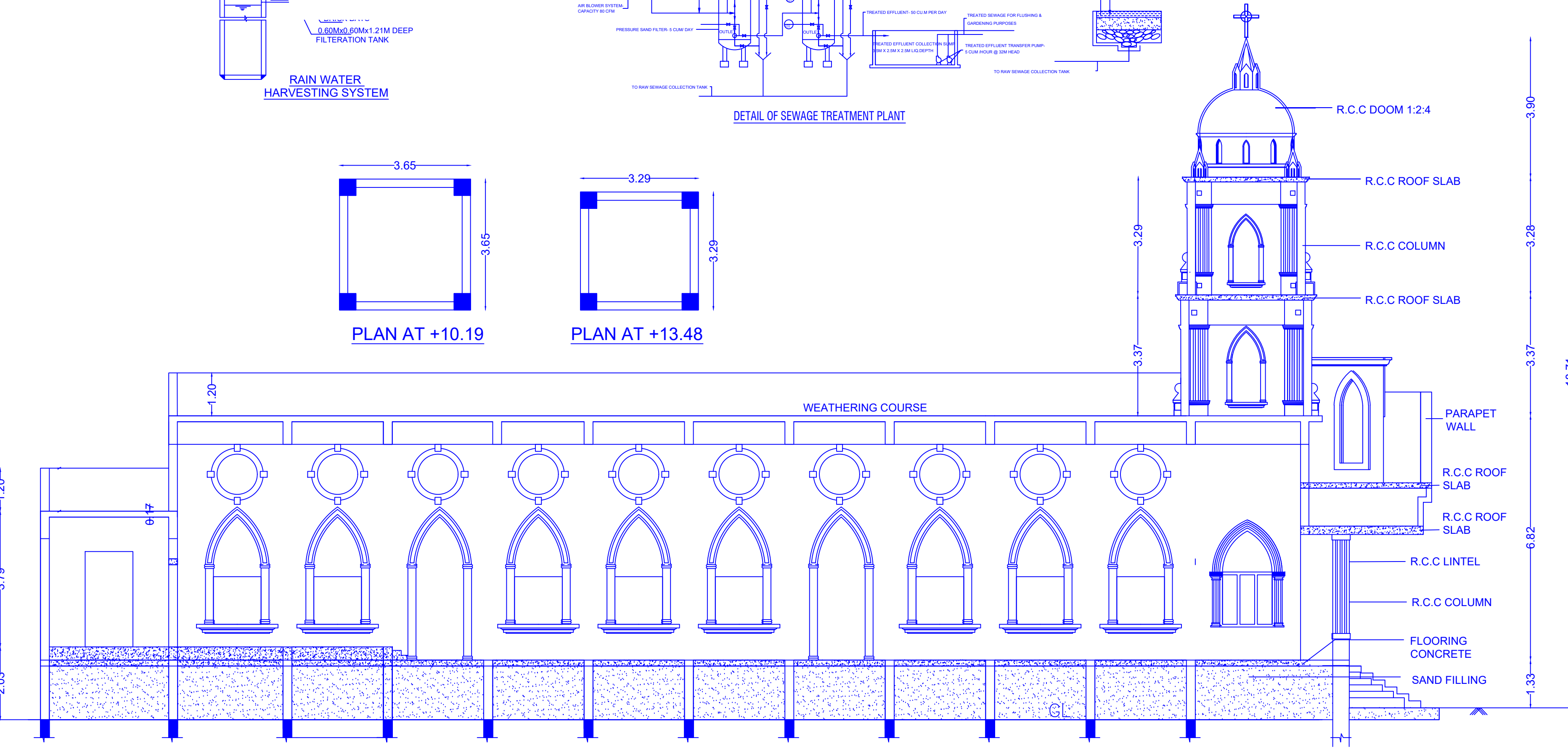
SECTION C-C
