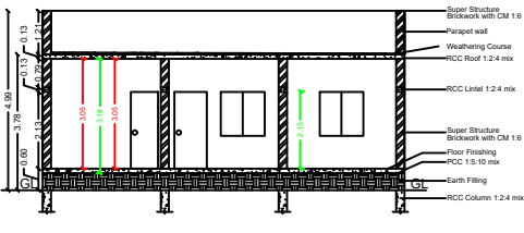
SECTION ON "VR"
