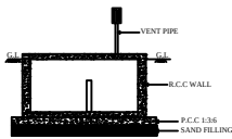
SECTION ON D-D
