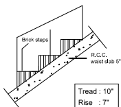
STAIRCASE DETAIL S-nts
