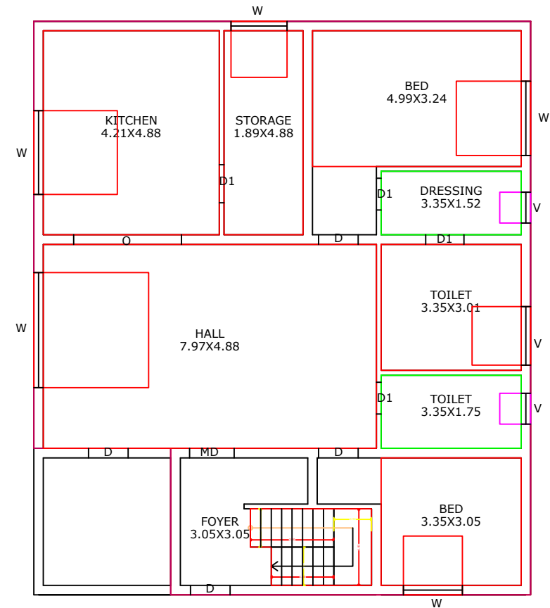
EXG FIRST FLOOR PLAN
