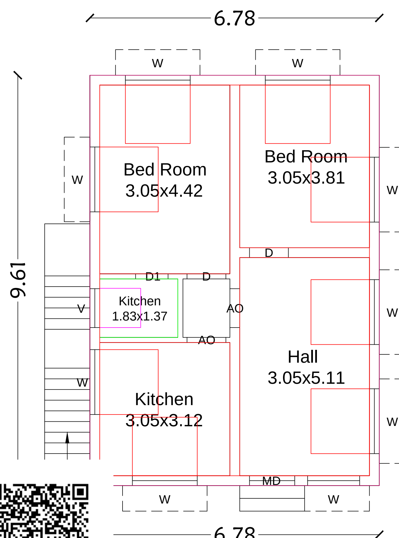
Ground Floor
