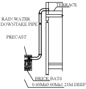
RAIN WATER DOWNTAKE PIPE
