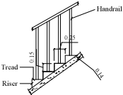
STAIRCASE DETAIL
