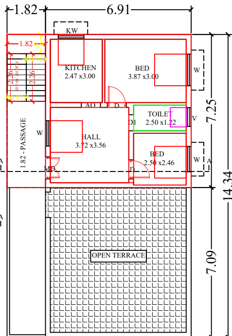
SECOND FLOOR PLAN (PROPOSED BUILDING)
