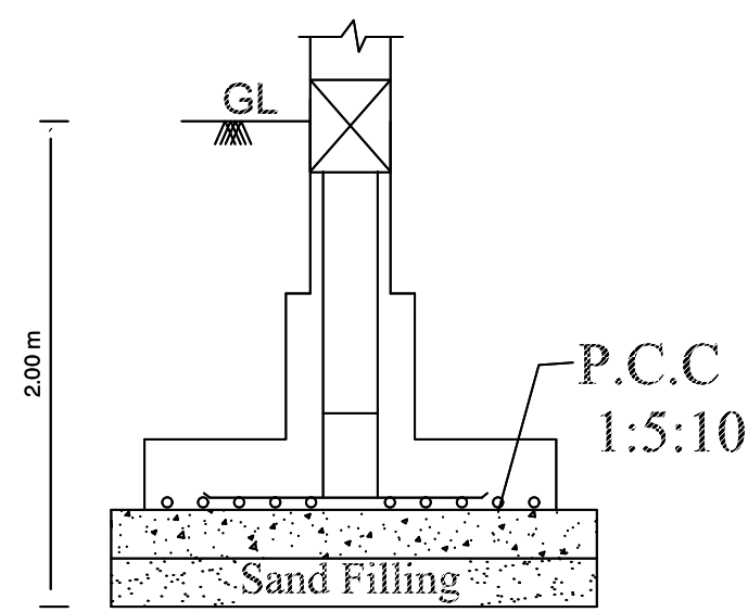
Isolated Footing -A (1.50X1.50) (Not to Scale)
