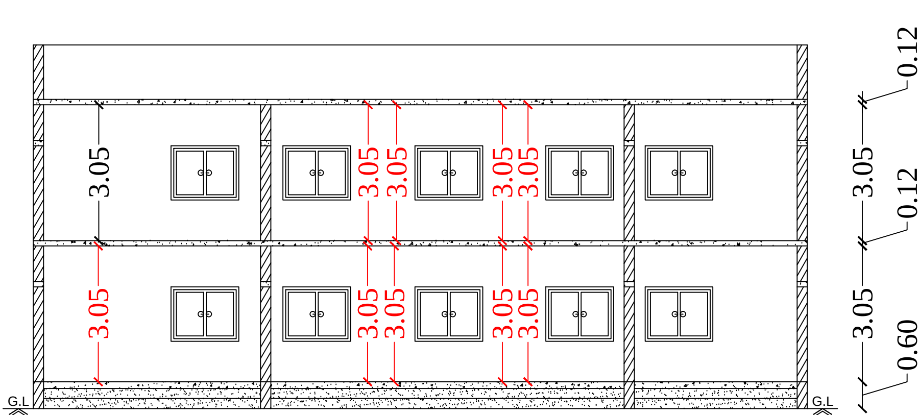
Section on-"AA"
