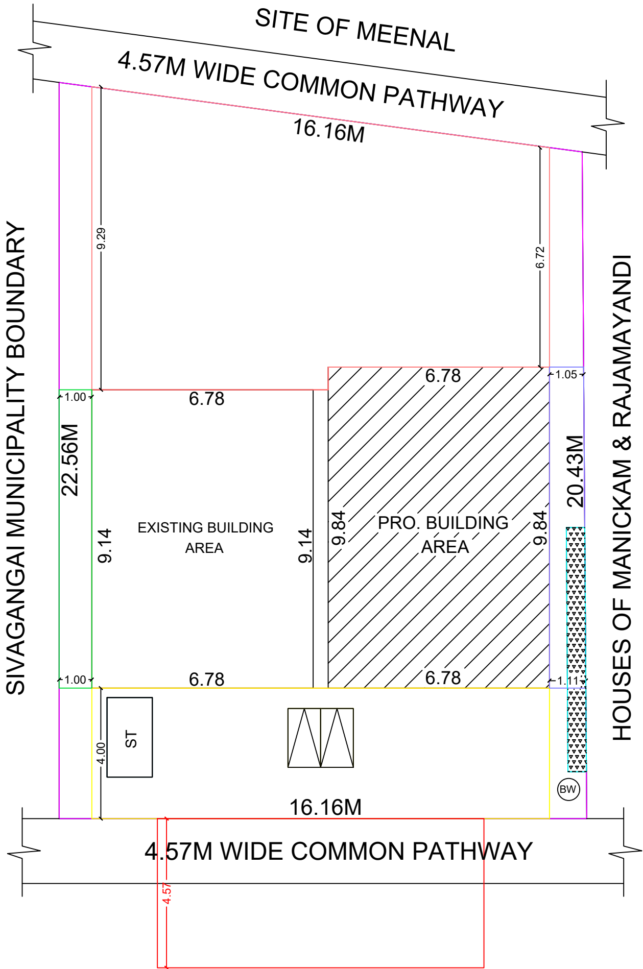
SITE PLAN
