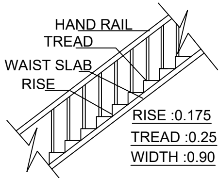
STAIRCASE DETAILS
