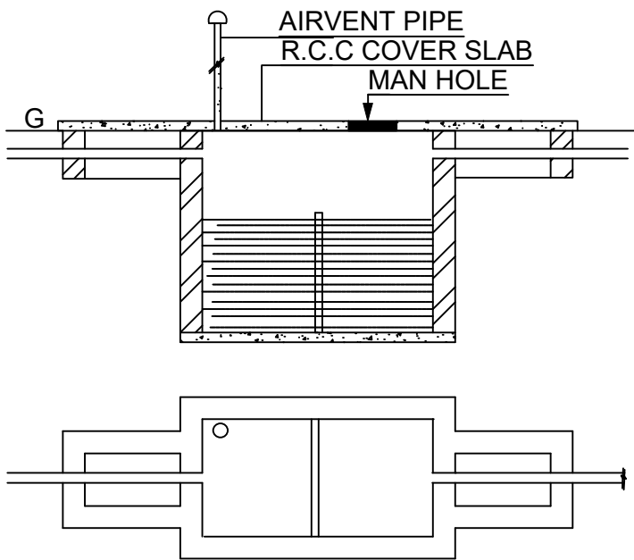
RAIN WATER HARVESTING
