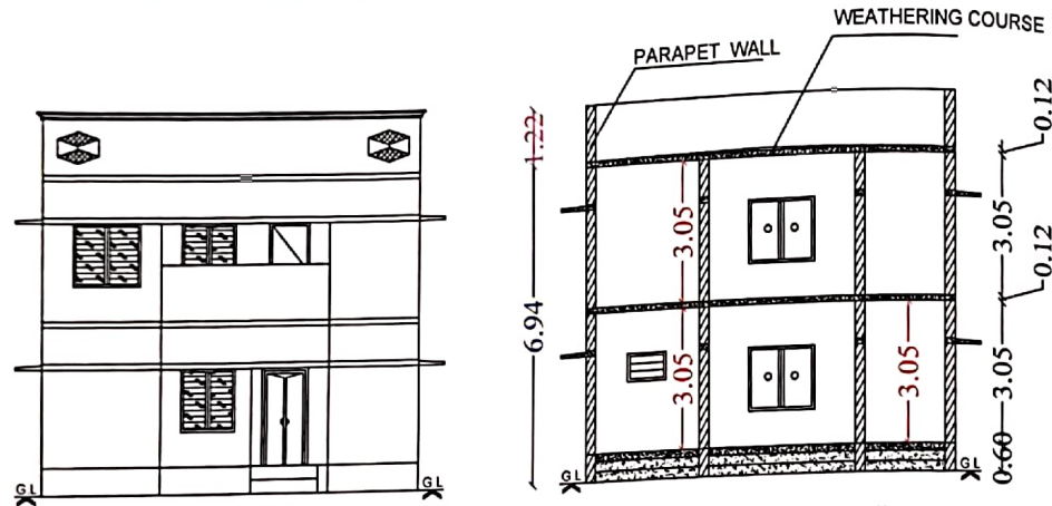
Section on-AA
