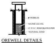
OREWELL DETAILS SCALE 1:100
