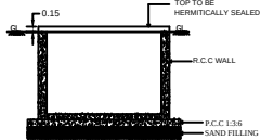
SECTION ON B-B SCALE 1:100
