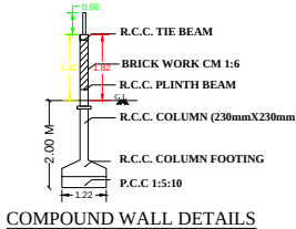
COMPOUND WALL DETAILS SCALE 1:100
