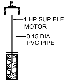
BORE WELL DETAILS
