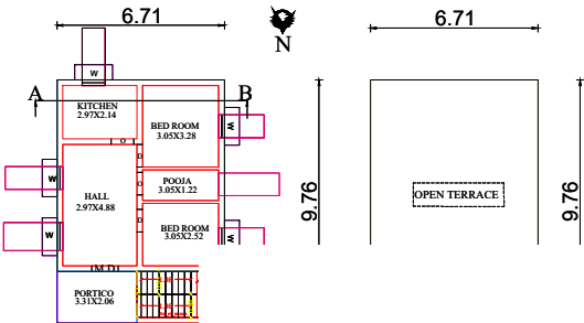
PROPOSED GRO FLOOR PLA
