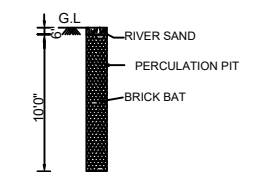
PERCULATION PIT
