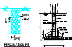
FOUNDATION DETAILS SCALE : 1:50
