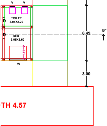
PRO. GROUND FLOOR PLAN
