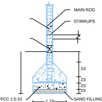
COLUMN DETAILS
