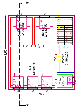
Pro.Ground Floor Plan
