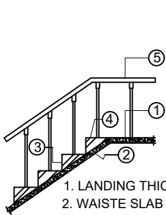
Staircase Details
