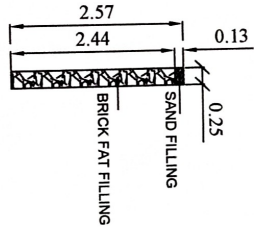
DETAILS OF PERCOLATION PIT
