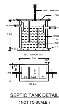
SEPTIC TANK DETAILS (NOT TO SCALE)
