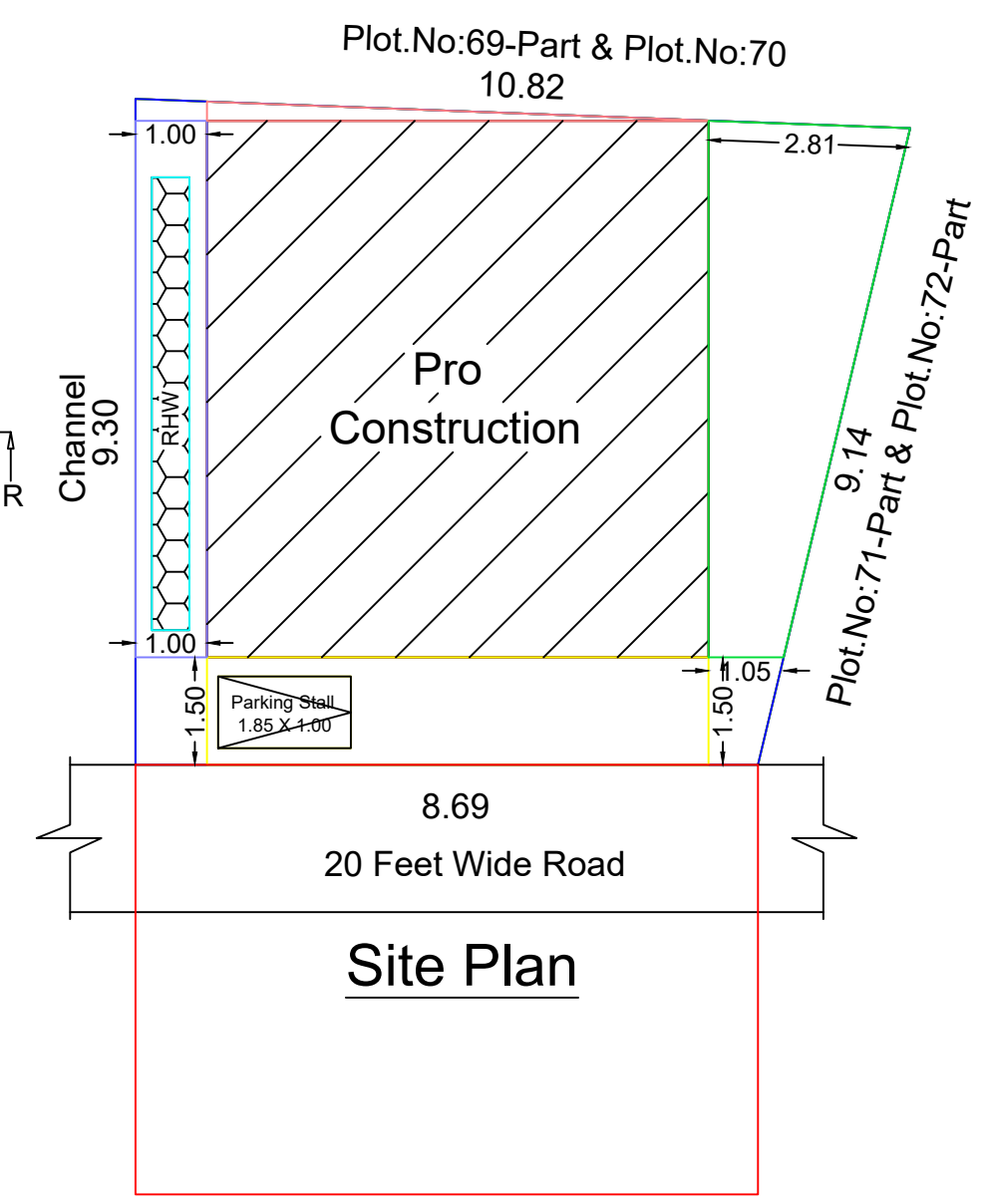
RAINWATER HARVESTING SYSTEM RWH_CAPACITY_L=2000
