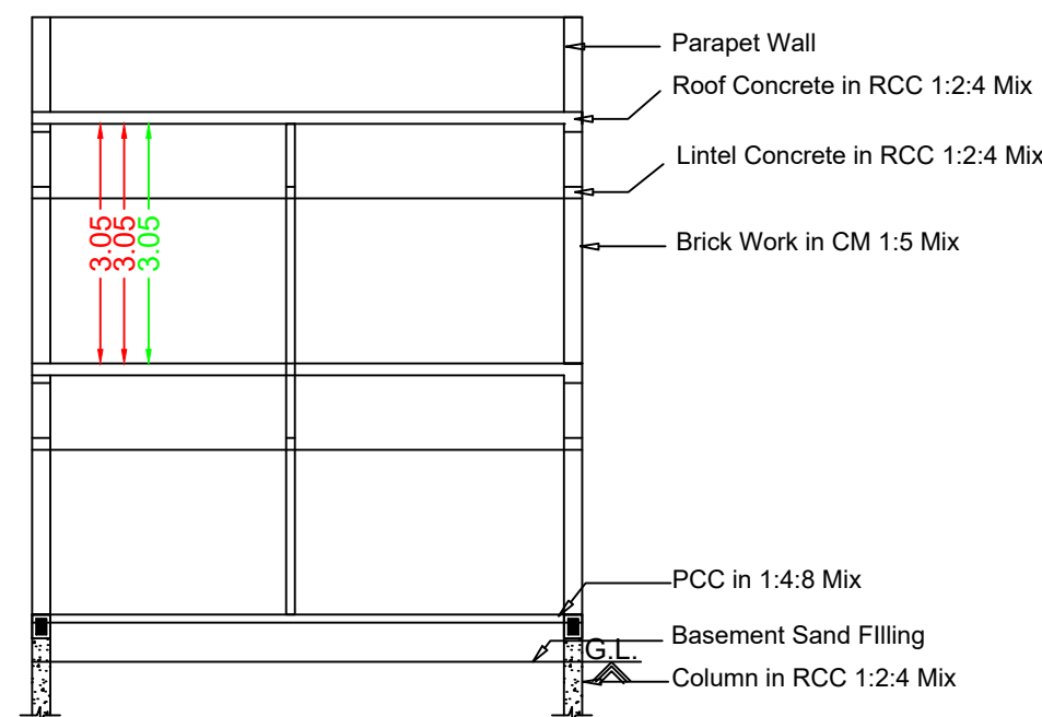
Section RR
