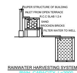
RAINWATER HARVESTING SYSTEM RWH_CAPACITY_L=2000
