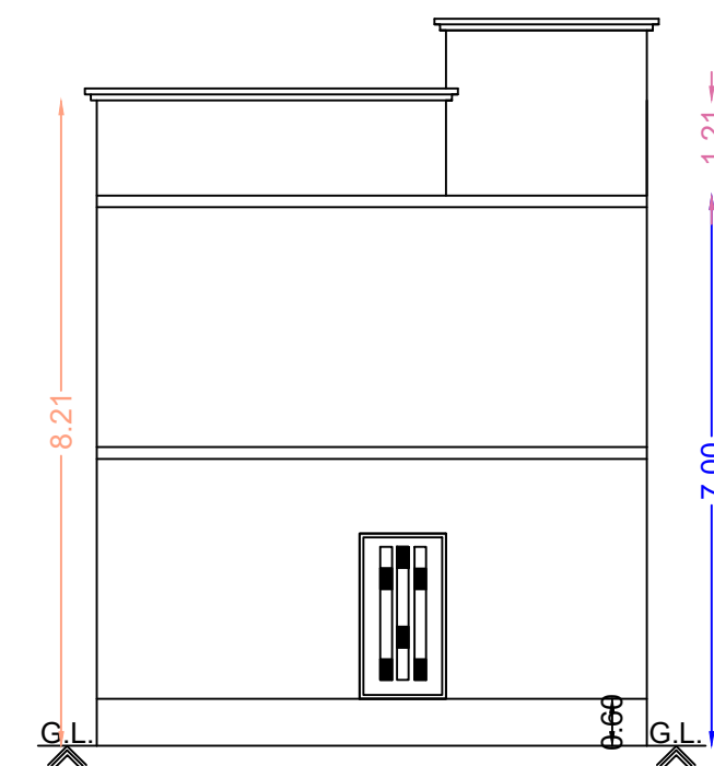
Front Elevation
